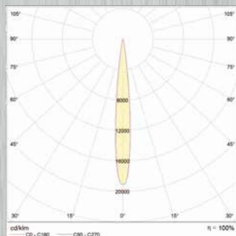
CURVA POLARE 3LED (SPOT) POLAR DIAGRAM 3LED (SPOT)
