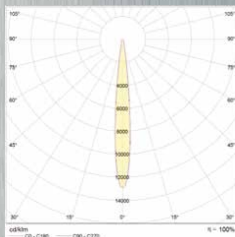
CURVA POLARE 5LED (WIDE+SPOT) POLAR DIAGRAM 5LED (WIDE+SPOT)
