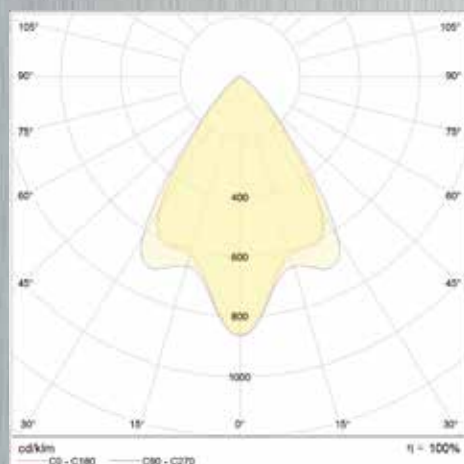
CURVA POLARE 2LED (WIDE) POLAR DIAGRAM 2LED (WIDE)
